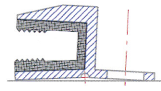
Figure 2: Alumero Laminat SECURITAS (End Clip)
