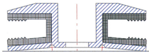
Figure 1: Alumero Laminat SECURITAS (Mid Clip)
